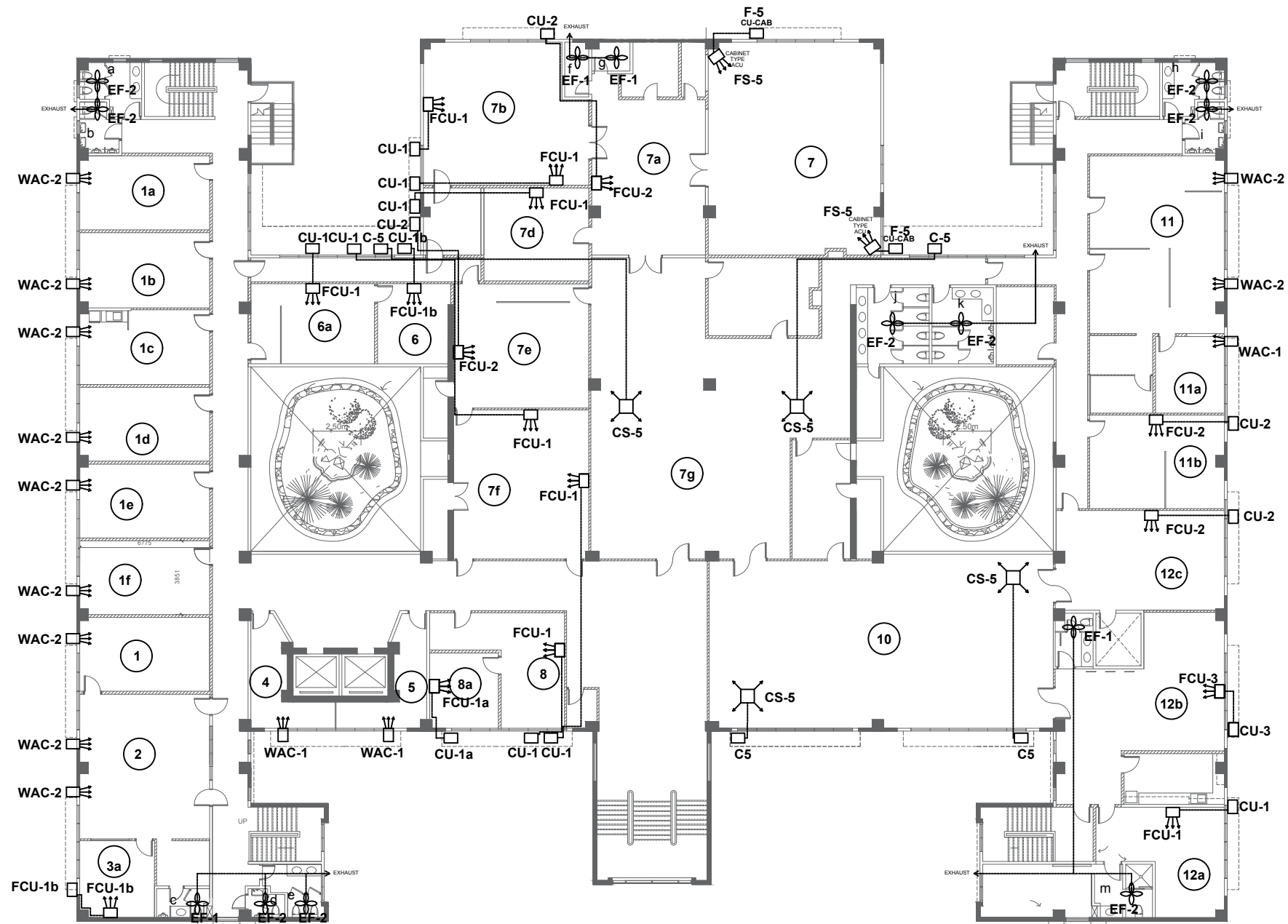
FOURTH FLOOR AIR CONDITIONING PLAN SCALE 1:150MTS.
