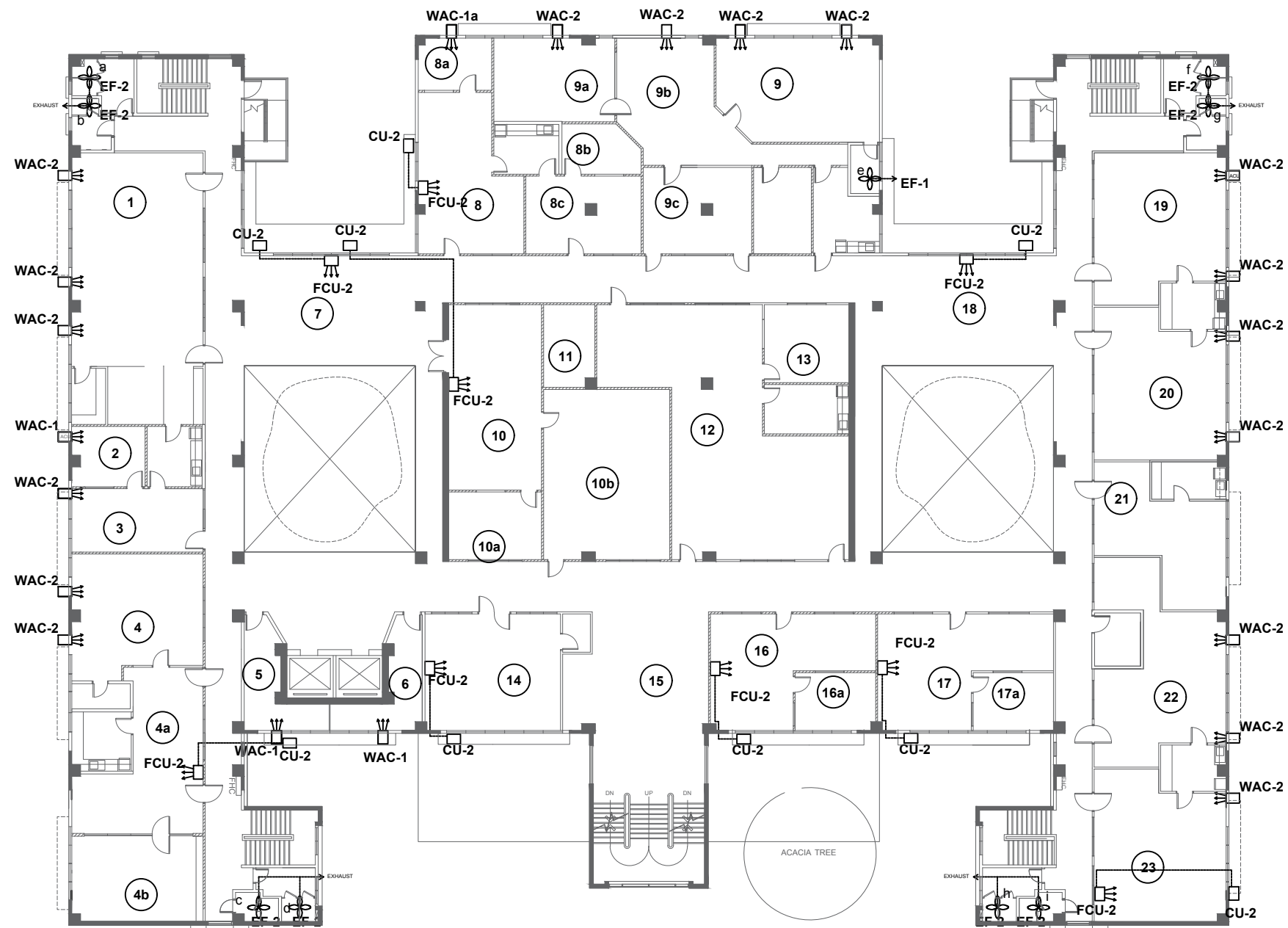
○ SECOND FLOOR AIR CONDITIONING PLAN SCALE 1:150MTS.
