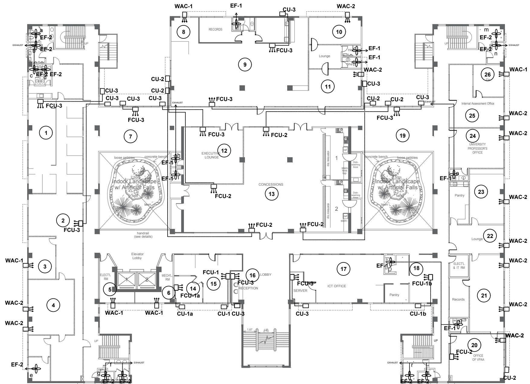
THIRD FLOOR AIR CONDITIONING PLAN SCALE 1:150M.TS.
