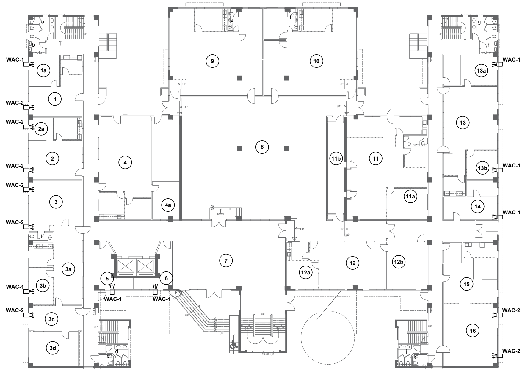
GROUND FLOOR AIR CONDITIONING PLAN SCALE 1:150MTS.
