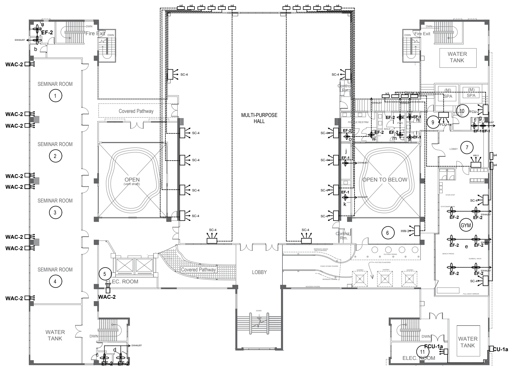
FIFTH FLOOR AIR CONDITIONING PLAN SCALE 1:150MTS.
